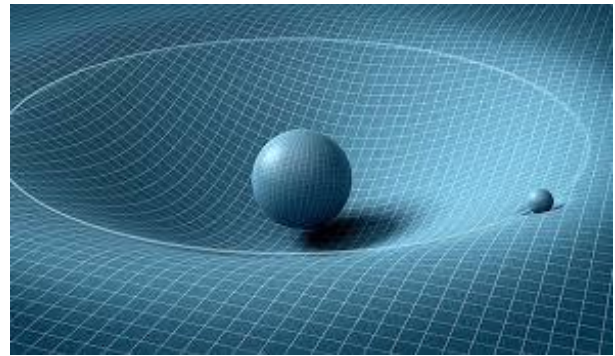
Figure ٣-١: An explanation of the concept of space-time curvature (gravity in modern physics)
